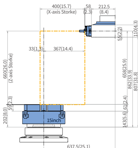
STRAIGHT MILLING HOLDER
