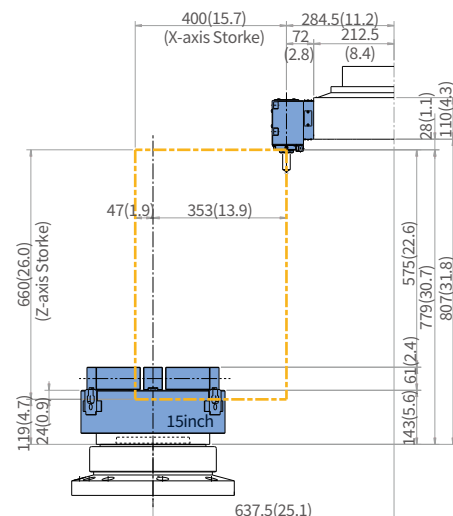
ANGULAR MILLING HOLDER
